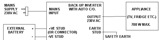
FIGURE 1 CONCEPT AND CONNECTION DIAGRAM.
